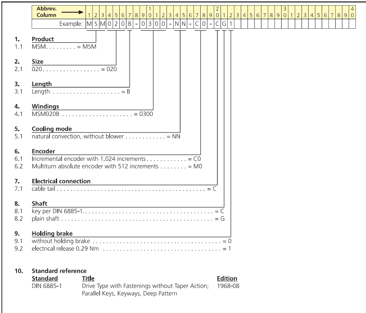
Fig. 8-1: Type code for motor MSM020B
