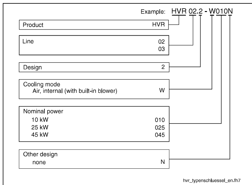
Fig. 4-7: Type code of power supply units HVR
