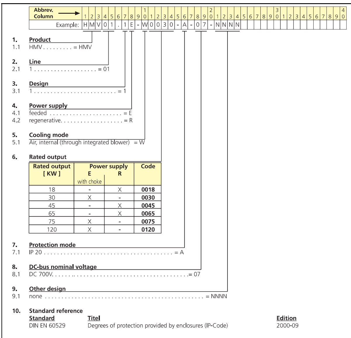
Fig. 4-1: Type code
