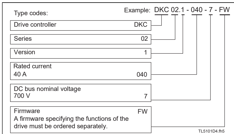
Fig. 4-8: DKC type code
