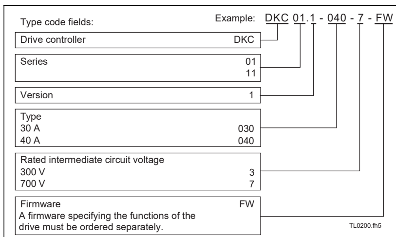
Fig. 4-10: DKC type code
